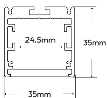
Luminaire Profile
